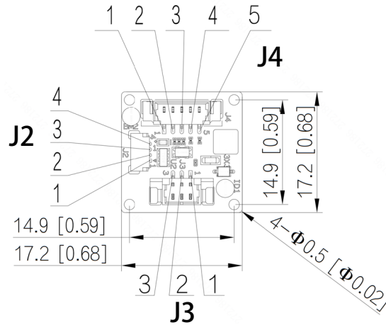
Figure 3-3Mini -CVBS expansion board (mm [inch])
